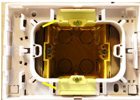
INSTALLATION ON UNI 502 SOCKET TYPE
